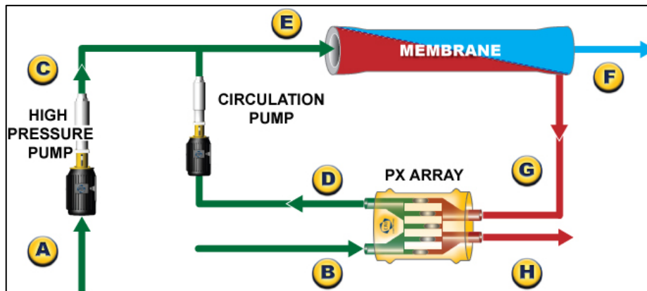
Figure 2 – Schematic Diagram of Hypothetical SWRO Train
