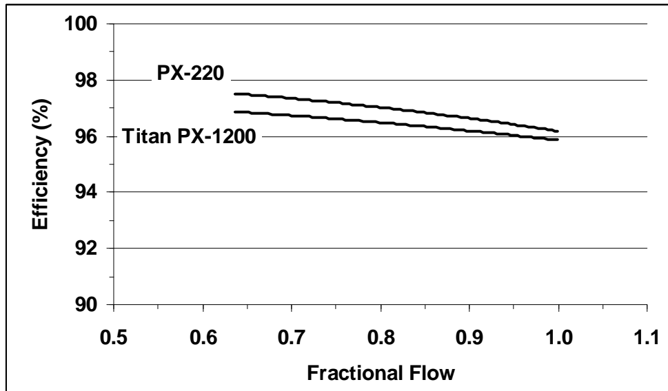
Figure 4 – Titan PX-1200 and PX-220 Efficiency on ERI Test Stand
